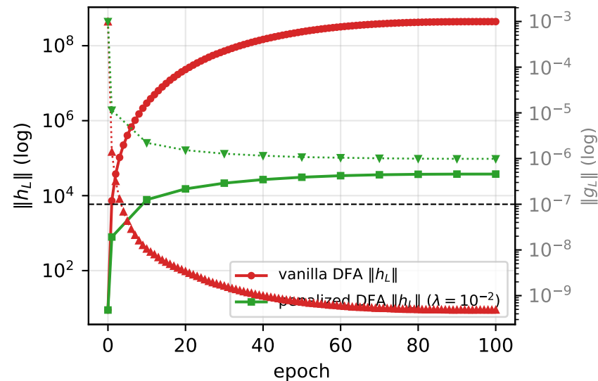
(a) penalty contains residual stream (4 OOM rescue)
