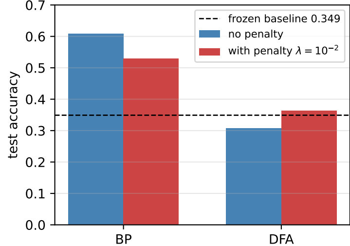
(c) BP+penalty 2 \times 2 control (BP-pen-cost -8pp; gap 17pp = credit quality)
