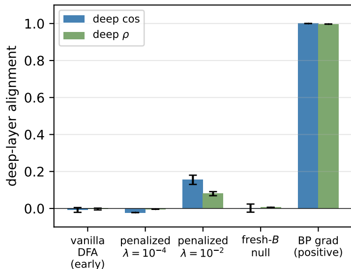
(b) two metrics agree across conditions (measurement vs random feedback)
