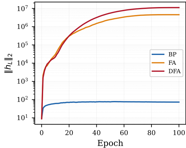
\|h_L\| (residual norm)
