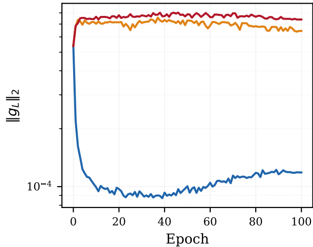
\|g_L\| (BP gradient at h_L )
