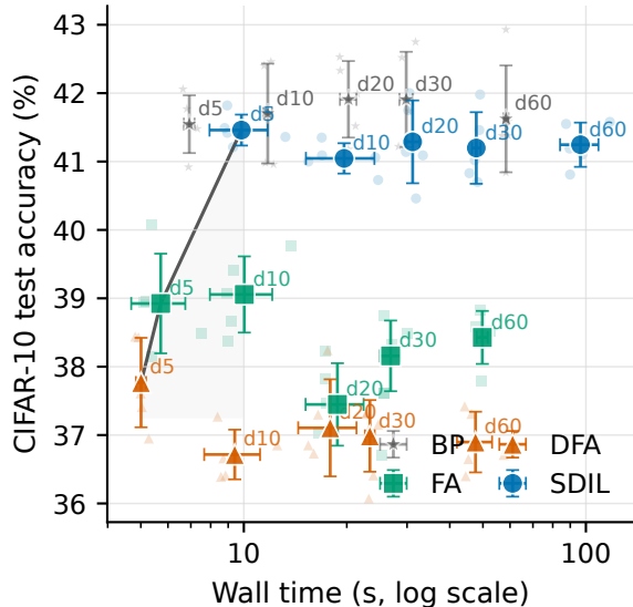
a Local-learning Pareto frontier
