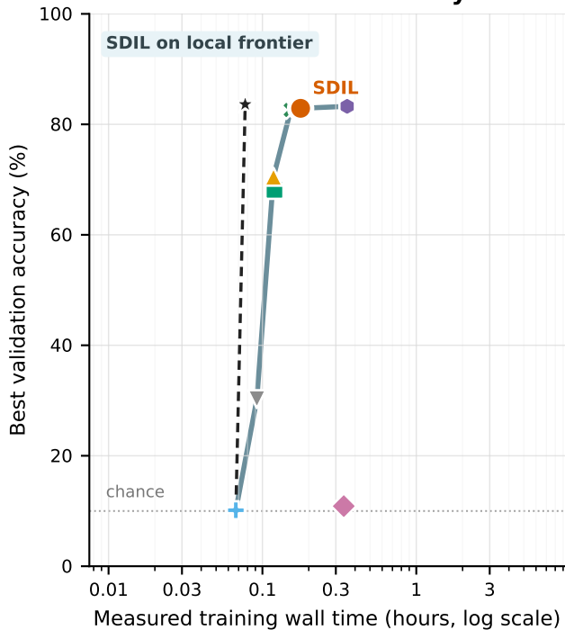
a miniCNN · 3 trainable layers
