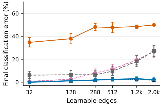
(a) Final-error growth 96% lower slope vs static calibration
