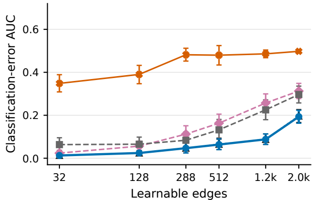
(b) Error-AUC growth Excess-growth slope eliminated
