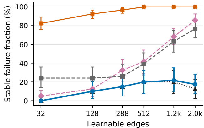
(c) Stable-failure growth 89% lower slope vs static calibration
