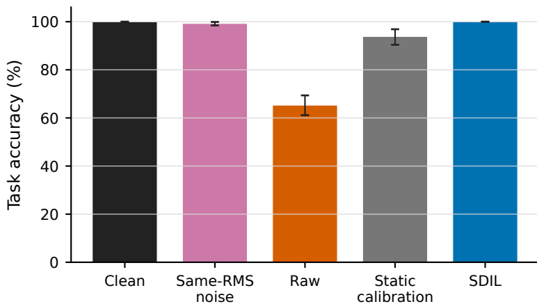
(c) Coupled learning · 32 edges 100% of clean gap recovered
